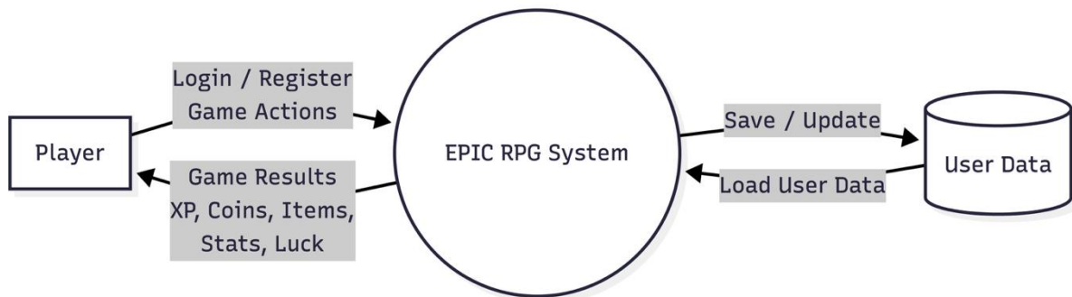
Figure 5.2 DFD-0
