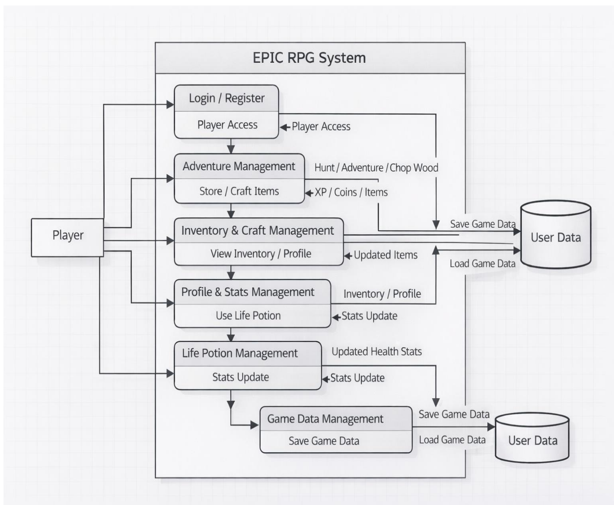
Figure 5.3 DFD Level-1
