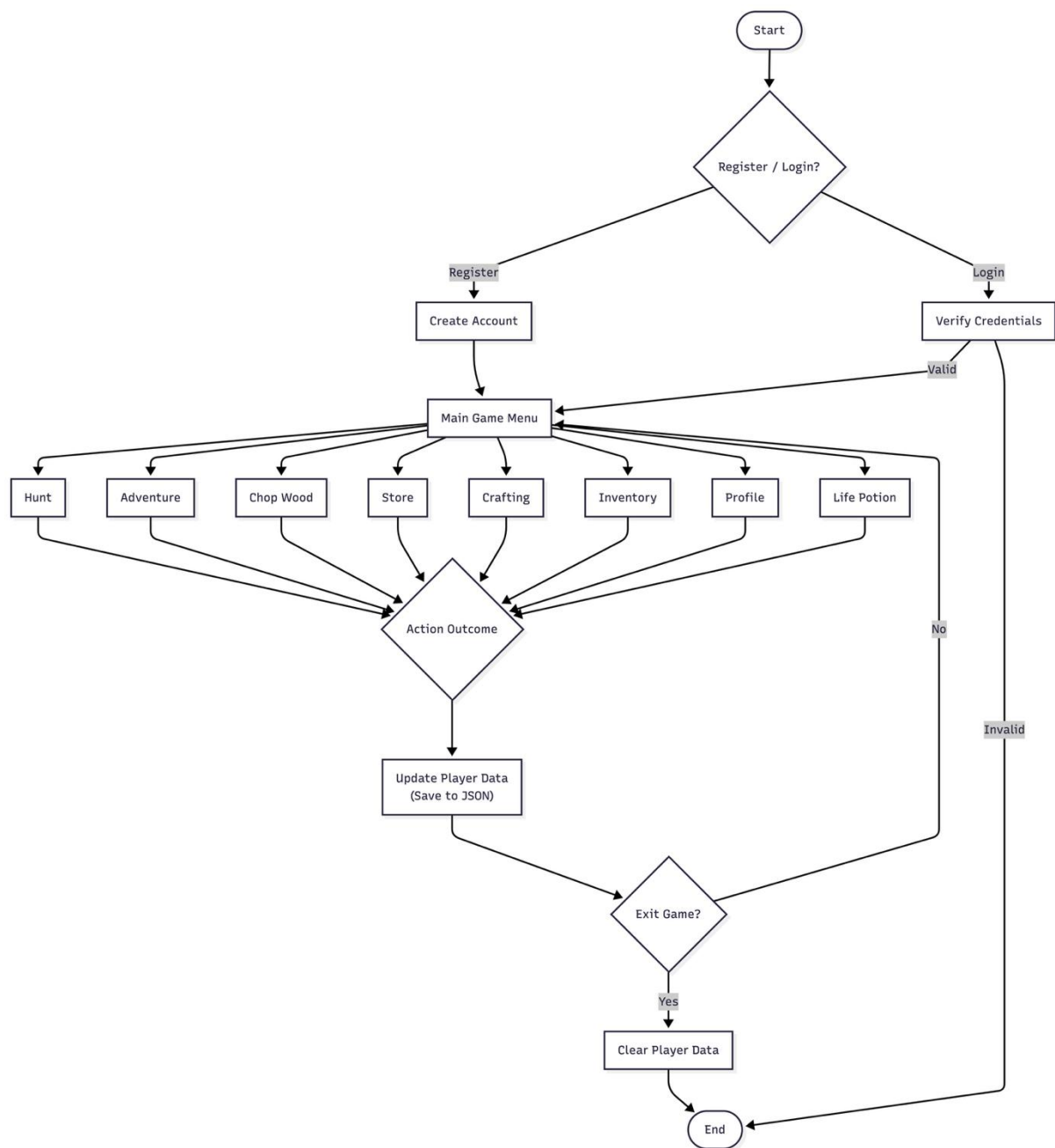
Figure 5.1 Flowchart:
